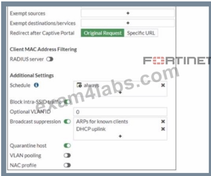
Firewall Policy
