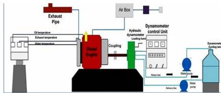
(a) Test engine schematic diagram
