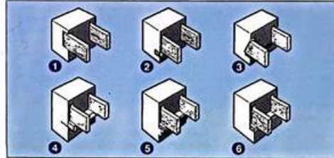
Figure 5.11 Sketches showing various arrangements for supporting floor joists: (1) joist with square end in pocket; (2) joist carried on wooden wall plate; (3) joist with splayed end in pocket; (4) joist carried on wooden wall plate carried on bracket; (5) joist carried on wooden wall plate on corbelled brickwork; (6) joist carried on wooden wall plate on a ledge formed by reducing the thickness of the wall.
