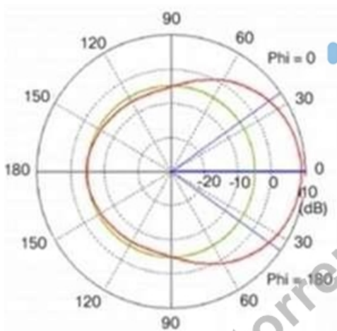
Antenna Azimuth Plane Pattern
