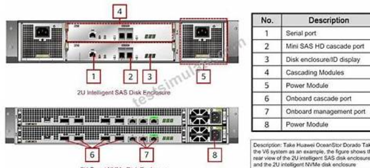
Disk enclosure rear view
