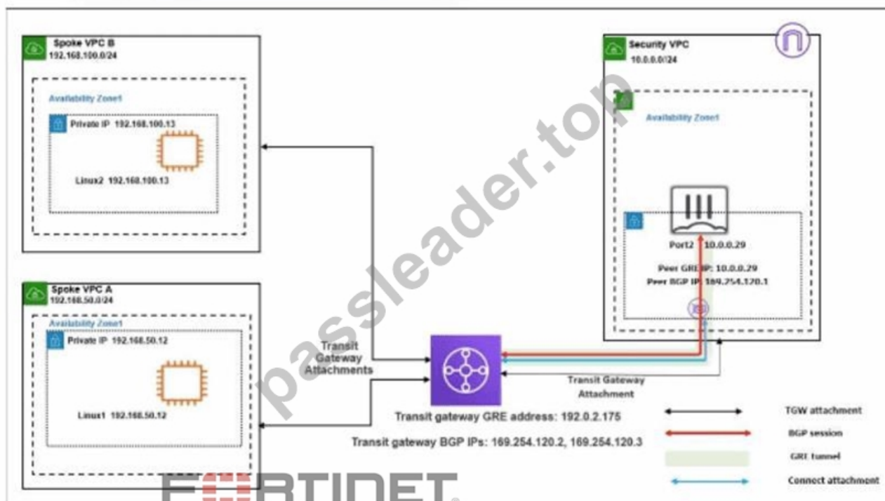
Network Topology
