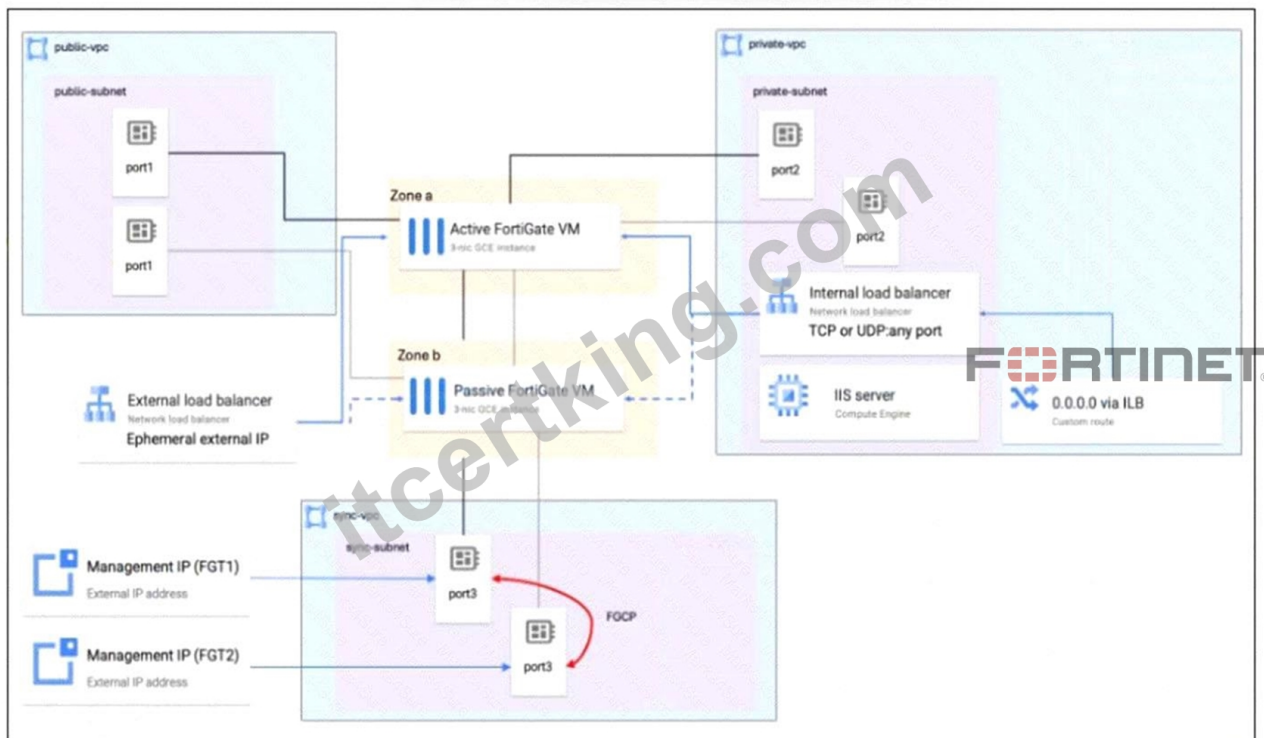
Active-passive HA environment
