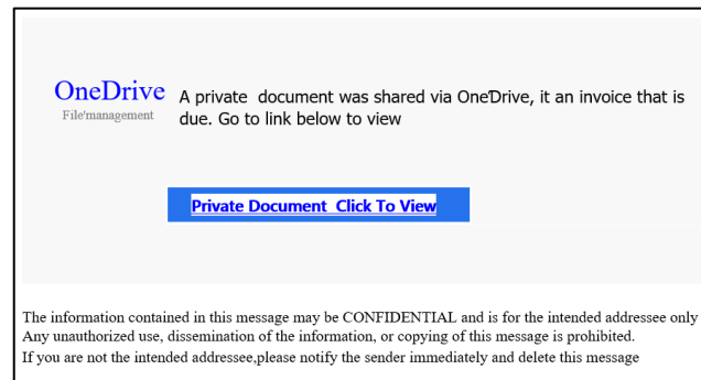
Figure 1. Phishing email
