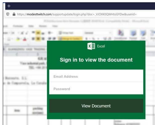
Figure 2: Phishing website
