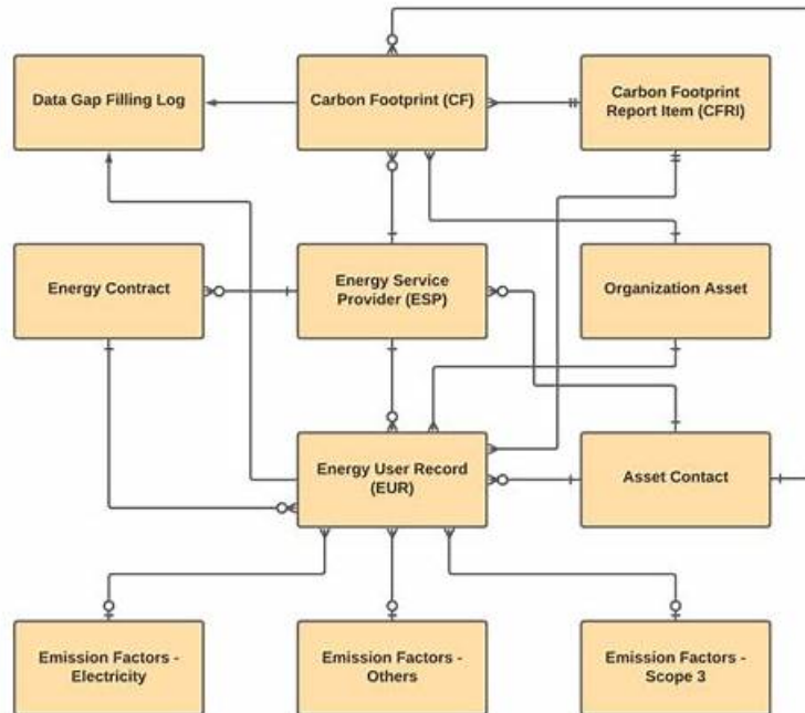
Salesforce Net Zero Cloud Entity Relationship Diagram
